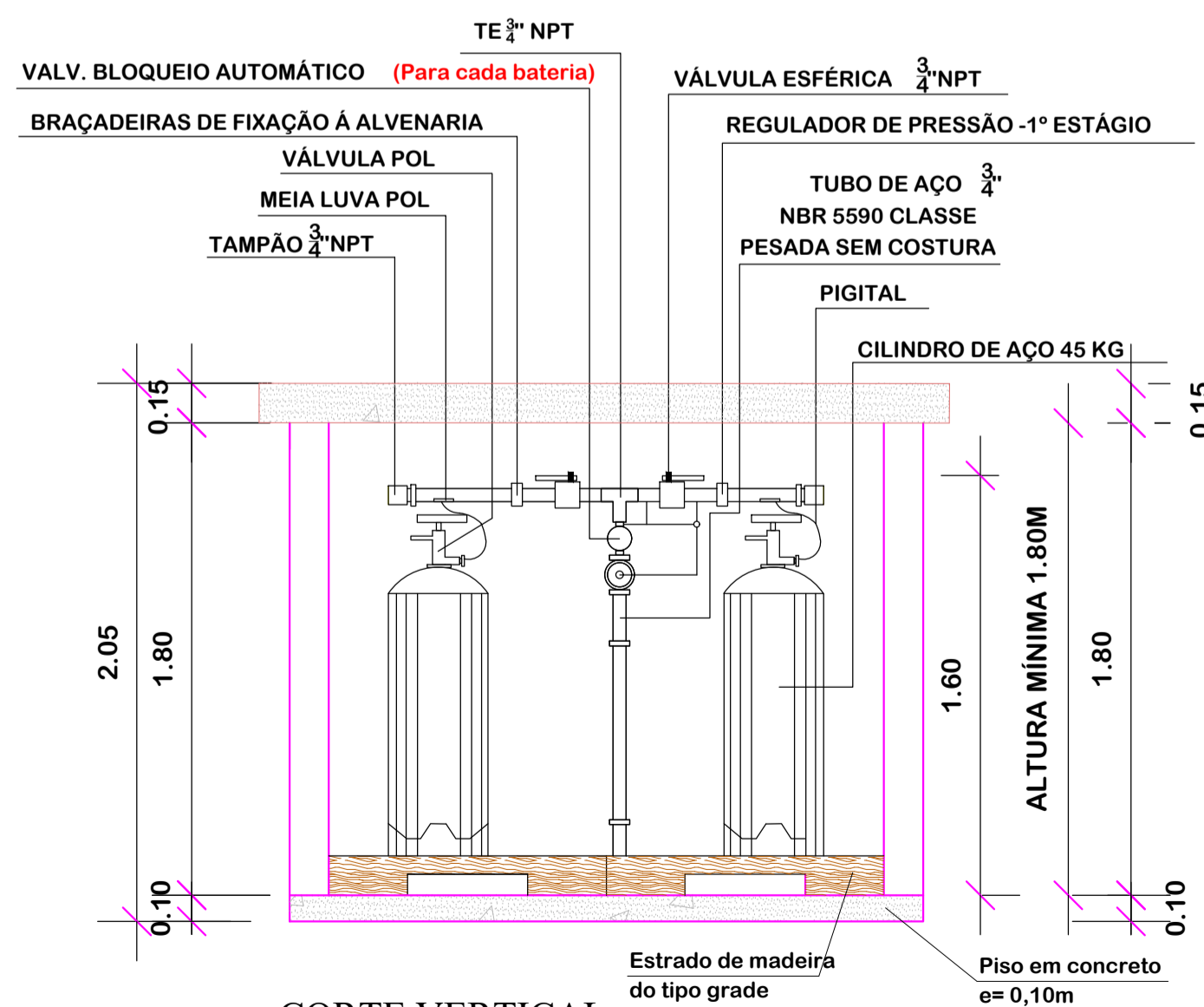
CORTE VERTICAL ESC:1/25
